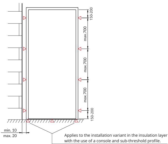
Optimal door and sidelight anchoring points
