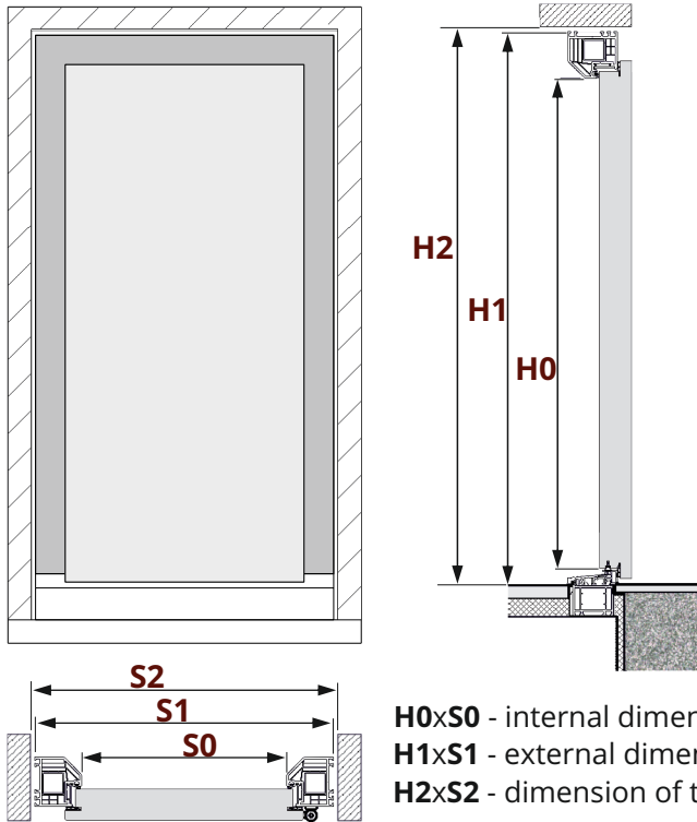
Door dimensioning diagram
