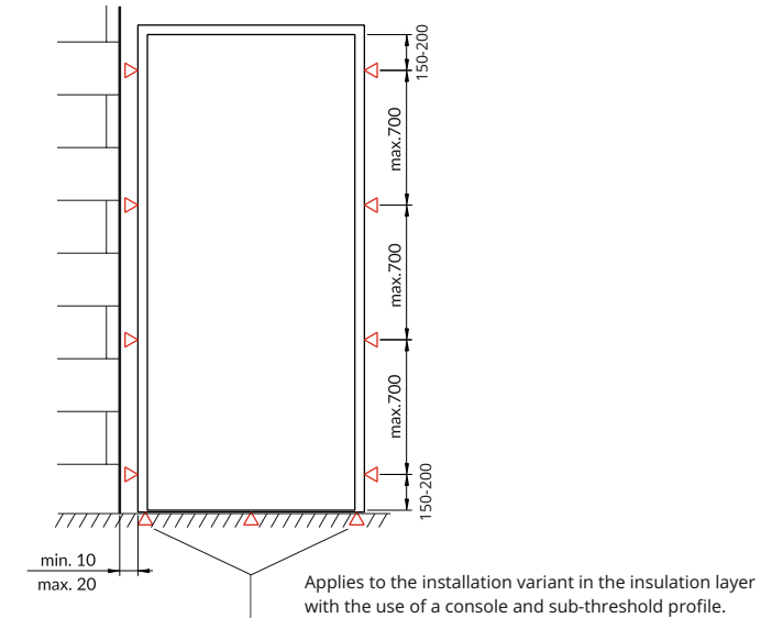
Optimal door and sidelight anchoring points
